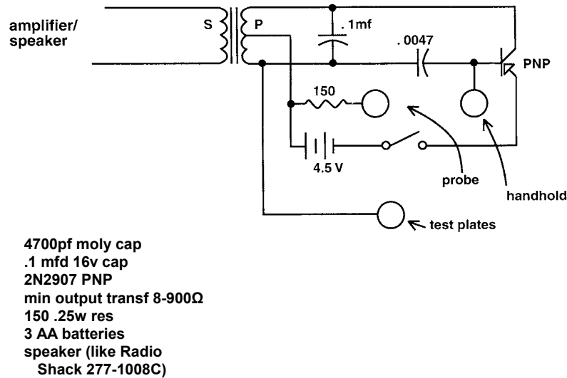
Fig. 79 Syncrometer schematic.
